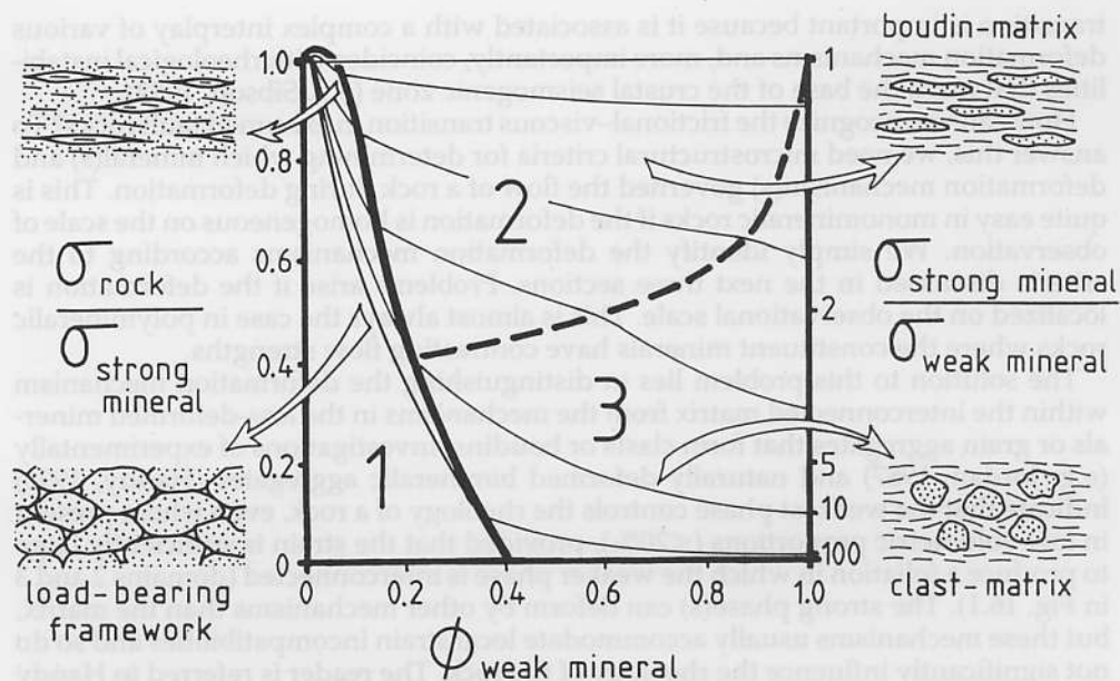
Figure 16.1 Diagram modified from Handy (1990) showing the strength of a biminerale rock as a function of the volume proportion of the weak mineral ( \phi_w ). The left-hand vertical axis indicates the normalized rock strength (strength of the stronger mineral set equal to one). The thick curve separates the load-bearing framework rheology (domain 1) from the matrix-controlled rheologies (domains 2 and 3). The thick dashed curve represents the gradational transition between boudin-matrix and clast-matrix rheologies (respectively, domains 2 and 3). The thin curves are contours of normalized rock strength at different mineral strength contrasts. They indicate the compositional dependence of rock strength for different mineral strength ratios shown on the right hand vertical axis. Arrows point to the dynamic steady-state microstructure for each domain (stippled: strong mineral; unstippled: weak mineral; lines: foliation). This diagram is based on microstructural and mechanical evidence from experimentally and naturally deformed rocks (see Handy, 1990 for further explanation).
