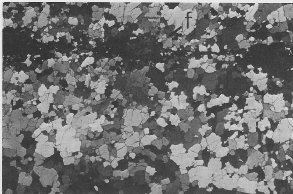
Figure 16.3 Post-tectonic grain growth has eliminated most direct microstructural evidence of previous viscous creep in this quartz-rich gneiss (compare with Fig. 16.2a and b). All traces of a shape fabric in quartz are gone, even though the boudinaged feldspar aggregates (marked with an f) suggest that the shear strain was very large. Annealing is incomplete, as evidenced by the locally non-linear grain boundaries and irregular grainsize. Amphibolite facies gneiss from the Strona-Ceneri Zone, Southern Alps (Handy, 1987). Frame dimensions: 9 \times 6 mm.
