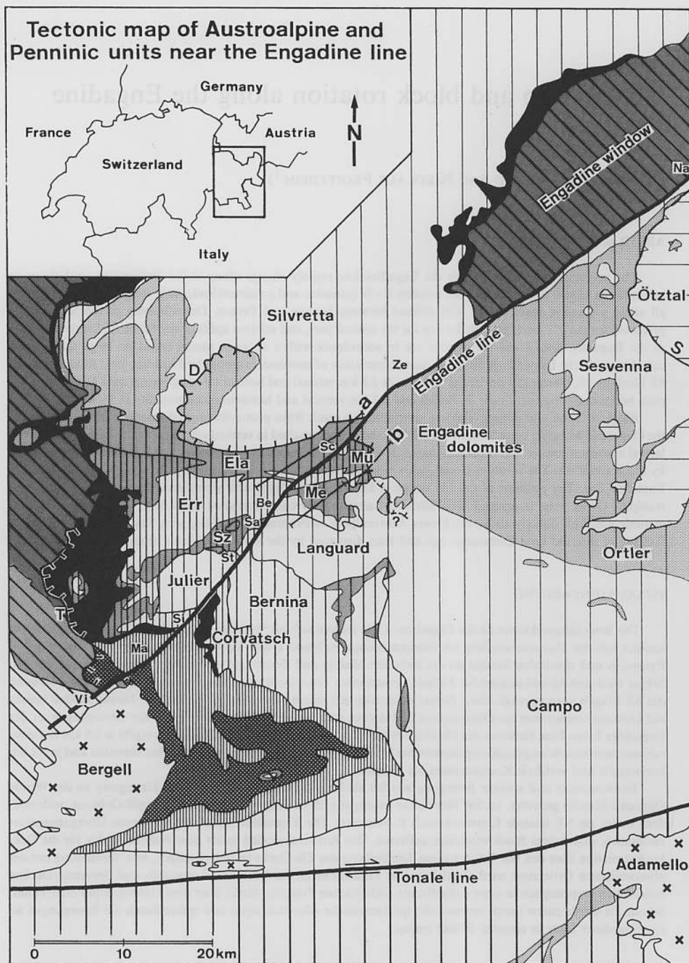
Fig. 1. Tectonic map of SE Switzerland. Profile traces refer to Fig. 7.
