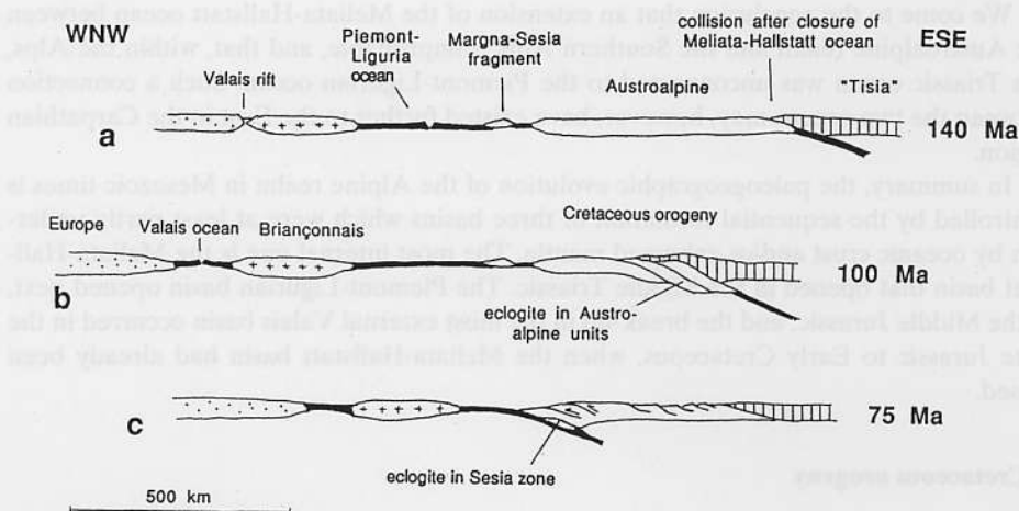
Fig. 4. Diagrammatic cross-sections showing the proposed sequence of events during the Cretaceous. Note that the sections are oriented WNW-ESE, parallel to the main direction of Cretaceous-age thrusting in the Austroalpine.
