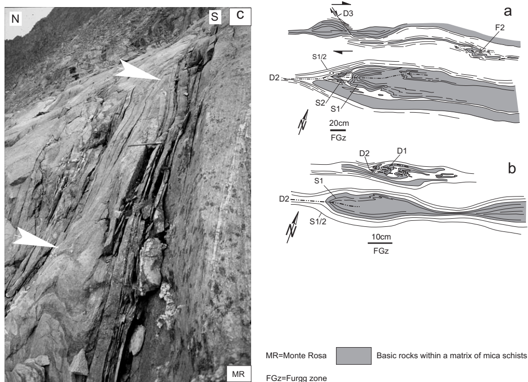
Fig. 6 Examples of fold-overprinting relationships, (a) and (b) in map view, (c) in profile view. (a) In fold hinges of D2 isoclinal folds S1 can be distinguished from S2 in mafic lithologies. D3 is indicated by asymmetric boudinage indicating top-ENE transport. Locality: western part of Alpi di Andolla. (b) Isoclinal D2 fold and evidence for D1 folding. Locality: western part of Alpi di Andolla. (c) Overprinting of an isoclinal D2 fold by an open D3 fold within orthogneiss from the Monte Rosa nappe. Upper arrow indicates a D2 fold hinge defined by S1; lower arrow indicates overprinting of both D2 fold limbs by an open D3 fold. Locality: SW of Lago Ciapivul.
