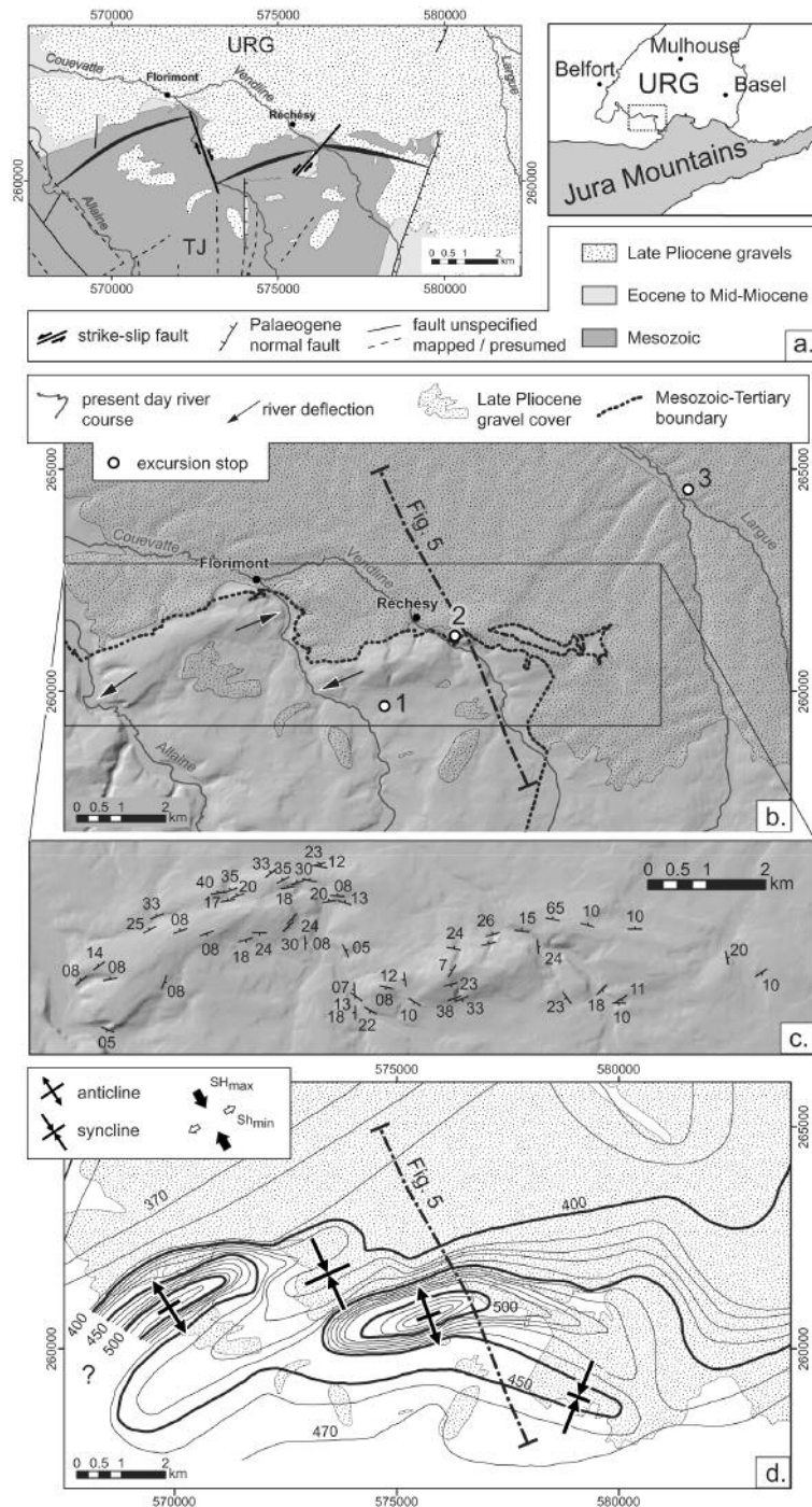
Fig. 4: (a) Simplified geological map of the area around the en-échelon aligned Florimont and Réchési anticlines at the Tabular Jura - URG boundary. (b) Shaded relief map illustrating the juvenile morphology of the two anticlines. Note the deflection of the Allaine and Coeuvalte rivers around the fold hinges. (c) Strike and dip of bedding planes measured in Mesozoic and Palaeogene sediments around the anticlines. (d) Contoured base of the Sundgau gravels (from Giamboni et al. 2004). Top left inset: recent stress field from a seismotectonic study of Kastrup et al. (2004). Figure modified after Ustaszewski & Schmid (in press). VSP-ASP convention 2006 excursion stops are indicated.
