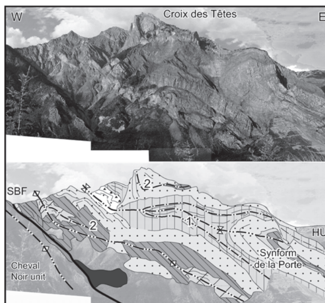
Fig. 8. Panorama of the southern part of the Subbriançonnais Unit (SBU) in the Croix de Têtes area. For patterns and symbols see legend enclosed in Fig. 4b. Note that the “Synforme de la Porte” looks like an antiform when seen from the Arc valley. This is due to intersection effects with the topography of its axial plane, dipping to the E, and of its fold axis, steeply plunging to the SE in the area of the photograph.
