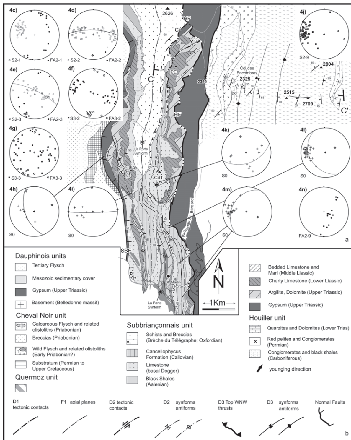
Fig. 4. a) Geological Map of southern part of the Subbriançonnais and of the Houiller units in the area between Grand Perron des Encombres, Pointe de la Masse (north) and the Croix des Têtes (south). See Fig. 1 for location. CV: Cicatrice de Varlossière; HF: For the other abbreviations see Fig. 1. b) Legend of the patterns, also valid for Figs. 7, 9, 10, 11 and 14, and, of the structural symbols, also valid for Figs. 6, 7, 8 and 9. c) to n) Equal area, lower hemisphere stereoplots. The first symbol besides the stereoplots indicates lineations, schistosity or fold axes of the different deformation phases (e.g. L1, L2, S0, S2, FA2). The second symbol (e.g. 1 in Fig. 4c) denotes the sub-area, where the data are from. See Fig. 3 for location of the sub-areas. Stereoplots d) and e) display best-fit poles for FA3, determined from folded S2 cleavages. Stereoplots h), i), k), l) & m) provide best-fit poles for FA2, determined from folded S0 cleavages.
