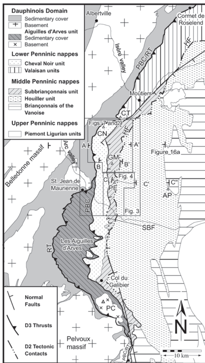
Fig. 1. Tectonic map of the Western Alps between Cornet de Roselend and Pelvoux Massif. Boxes indicate areas covered by Figs. 3, 4, 7 and 9. HF: Houiller frontal thrust; PBC: Penninic Basal contact; RT: Roselend thrust; SBF: Subbriançonnais front (mostly overprinted by normal faulting); AP: Aiguille de Péclet; GM: Aiguilles de la Grande Moendaz; PC: Pics de Combeynot; PE: Grand Perron des Encombres.
