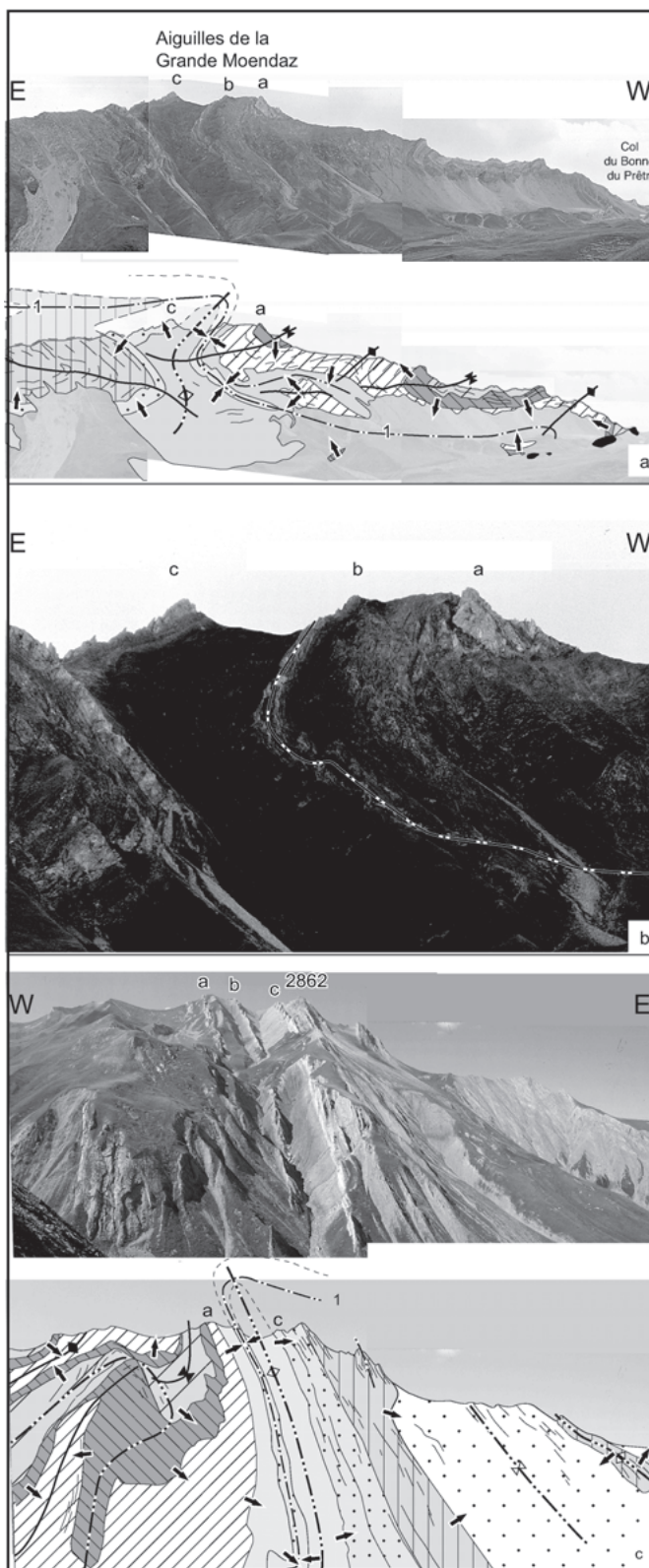
Fig. 11. Panoramic views of (a & b) northern and (c) southern wall of the Grande Moendaz (compare with Fig. 7 & profile B-B' of Fig. 10b). For patterns and symbols see legend given in Fig. 4b.
