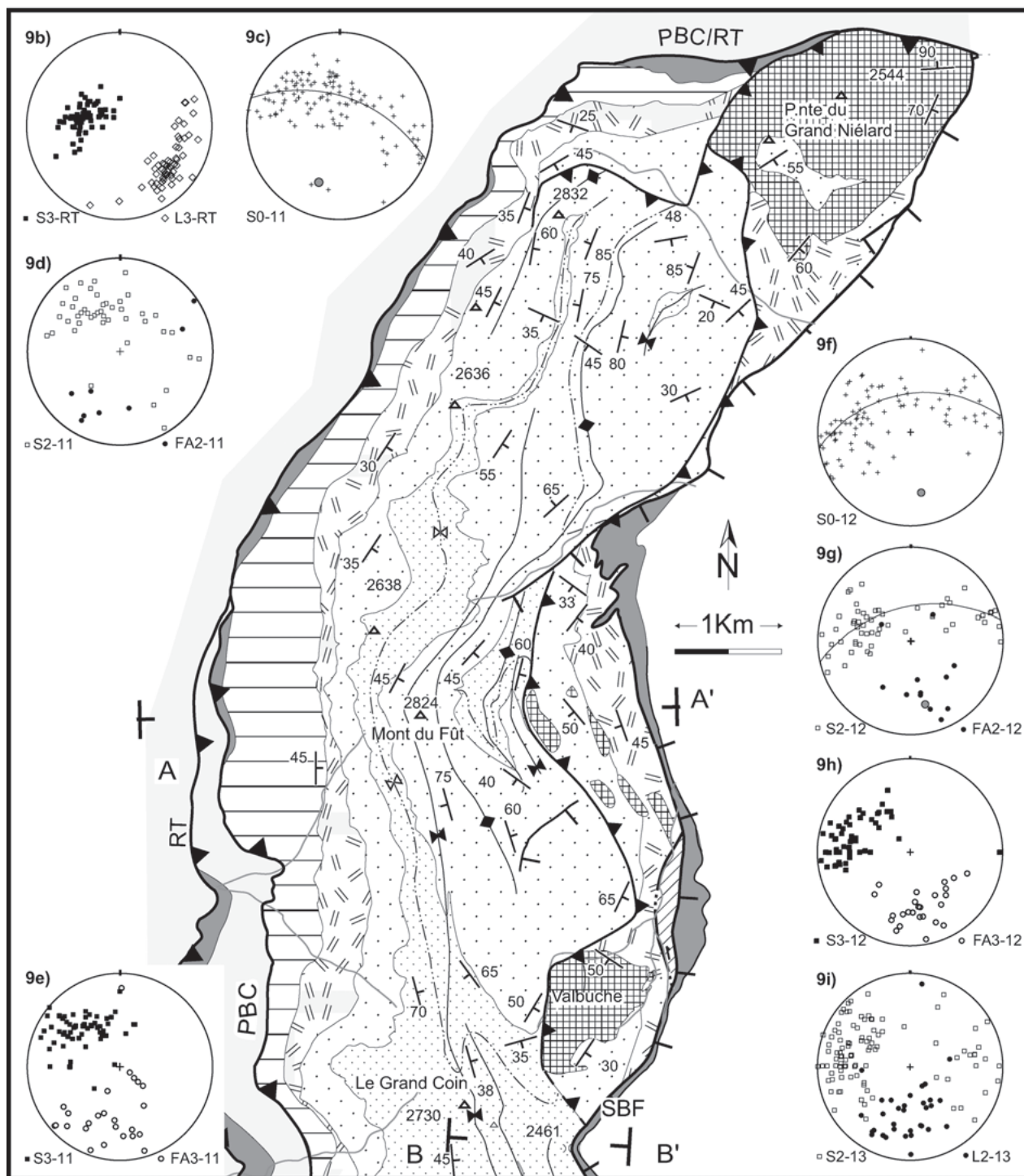
Fig. 9. Geological Map of the Cheval Noir Unit (CNU) between Niélard (north) and Le Grand Coin (south), see Fig. 1 for location, and for tectonic letter symbols. See legend given in Fig. 4b.
