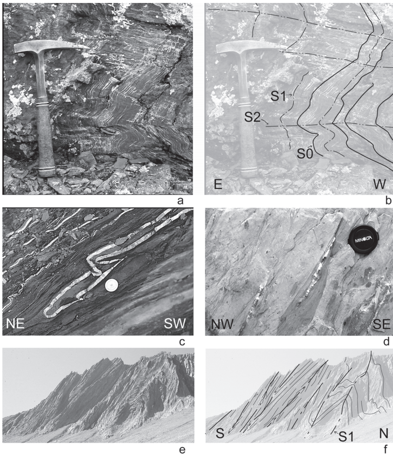
Fig. 2. Field photographs illustrating poly-phase deformation.
