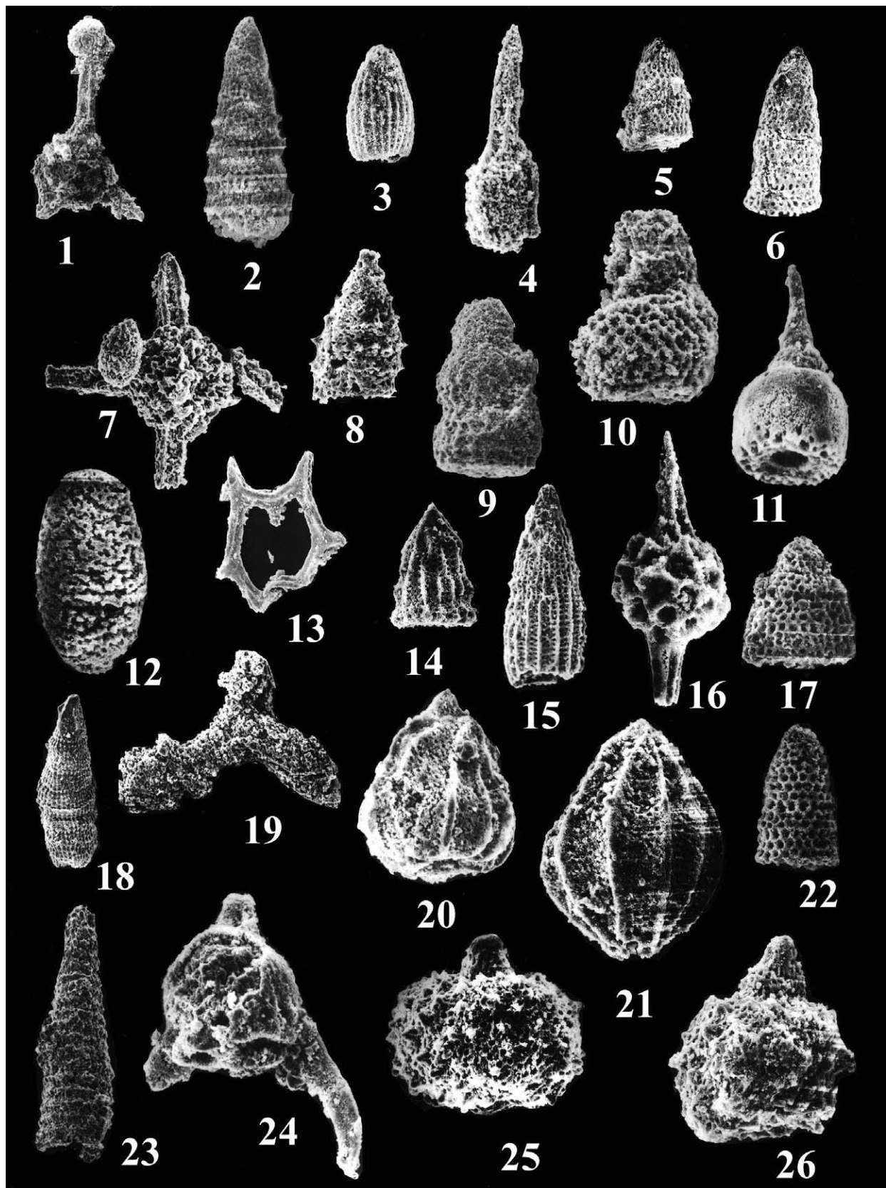
Plate 1 - 1. Acaeniotylopsis ? sp., NĐ 41, x100; 2. Amphipyndax ? sp., NĐ 47, x200; 3. Archaeodictyomitra sp., NĐ 43, x200; 4. Archaeospongoprimum ? sp., NĐ 42, x200; 5. Dictyomitrella ? sp., NĐ 43, x 200; 6. Dictyomitrella sp., NĐ 44, x 100; 7. Emiluvia sp., NĐ 41, x100; 8. Eoxitus sp. cf. E. hungaricus Kozur, NĐ 44, x300; 9. Eucyrtidiellum sp., NĐ 47, x200; 10. Eucyrtidiellum sp. cf. E. quinquatum Takemura, NĐ 47, x200; 11. Eucyrtidiellum unumaense unumaense (Yao), NĐ 45, x300; 12. Guexella ? sp., NĐ 41, x150; 13. Hexasaturnalis hexagonus (Yao), NĐ 46, x300; 14. Hsuum sp., NĐ 46, x200; 15. Hsuum sp. cf. H. matsuokai Isozaki and Matsuda, NĐ 44, x150; 16. Pantanellium sp. cf. P. riedeli Pessagno, NĐ 45, x300; 17. Parahsuum ? sp., NĐ 46, x300; 18. Parahsuum cruciferum Takemura, NĐ 44, x100; 19. Paronaella sp., NĐ 41, x100; 20. Protunuma sp. cf. P. lanosus Ošvoldova, NĐ 45, x300; 21. Protunuma turbo Matsuoka, NĐ 45, x300; 22. Pseudodictyomitrella hexagonata (Heitzer), NĐ 41, x200; 23. Ristola sp. cf. R. praemirifusus Baumgartner and Bartolini, NĐ 41, x100; 24. Saitoum levium De Wever, NĐ 45, x300; 25. Sethocapsa sp., NĐ 45, x300; 26. Sethocapsa funatoensis Aita, NĐ 45, x300.
