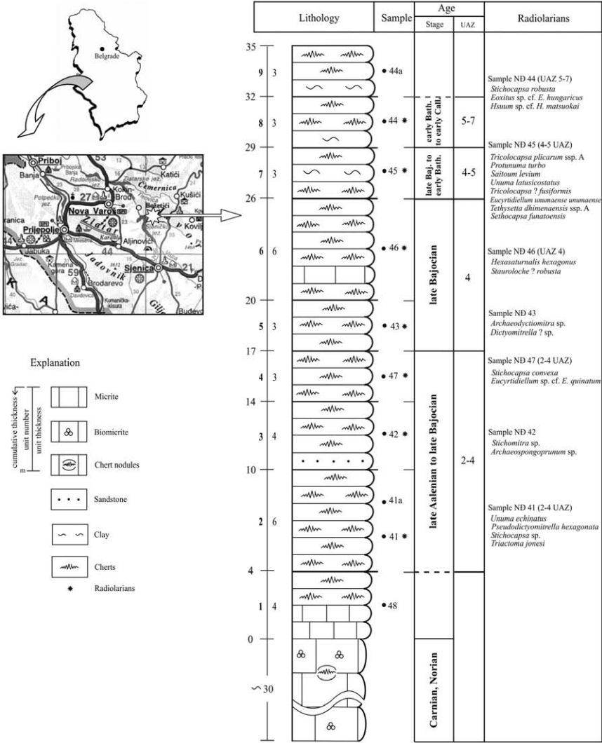
Fig 1 - Location and lithostratigraphic column of the Pavlovića Brod section, showing the principal radiolarian markers; UAZ after Baumgartner et al. (1995b).
