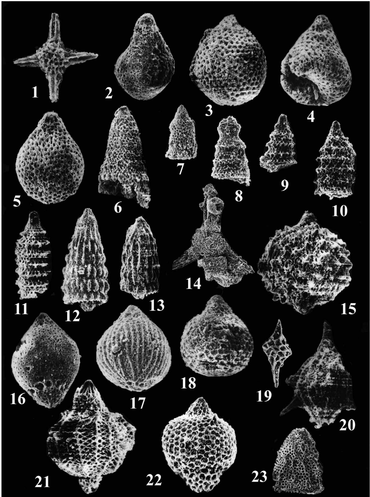
Plate 2 - 1. Stauroloche ? robusta Rüst, NĐ 46, x300; 2. Stichocapsa convexa Yao, NĐ 47 x 300; 3. Stichocapsa sp., NĐ 41, x 300; 4. Stichocapsa sp. cf. S. japonica Yao, NĐ 45, x300; 5. Stichocapsa robusta Matsuoka, NĐ 44, x300; 6. Stichomitra sp., NĐ 42, x200; 7. Stichomitra sp. cf. S. tairai Aita, x200; 8. Stichomitra ? takanoensis gr. Aita, NĐ 45, x200; 9., 10. Tethyssetta dhimenaensis s.l. (Baumgartner), NĐ 45, x200; 11. Tethyssetta dhimenaensis ssp. A (Baumgartner et al.), NĐ 45, x200; 12. Transhsuum sp. cf. T. brevicostatum gr. (Ošvoldova), NĐ 45, x200; 13. Transhsuum sp. cf. T. maxwelli gr. (Pessagno), NĐ 45, x200; 14. Triactoma jonesi (Pessagno), NĐ 41, x100; 15. Tricolocapsa sp. cf. T. formosa Chiari, Marcucci and Prella, NĐ 45, x300; 16. Tricolocapsa ? fusiformis Yao, NĐ 45, x300; 17. Tricolocapsa plicarum ssp. A Baumgartner et al., NĐ 45, x300; 18. Tricolocapsa ? yaoi (Kozur), NĐ 45, x300; 19. Trillus sp., NĐ 46, x200; 20. Unuma echinatus Ichikawa et Yao, NĐ 41, x100; 21. Unuma latusicostatus (Aita), NĐ 45, x300; 22. Williriedellum sp. cf. W. carpathicum Dumitrica, NĐ 45, x270; 23. Xitus sp., NĐ 44, x200.
