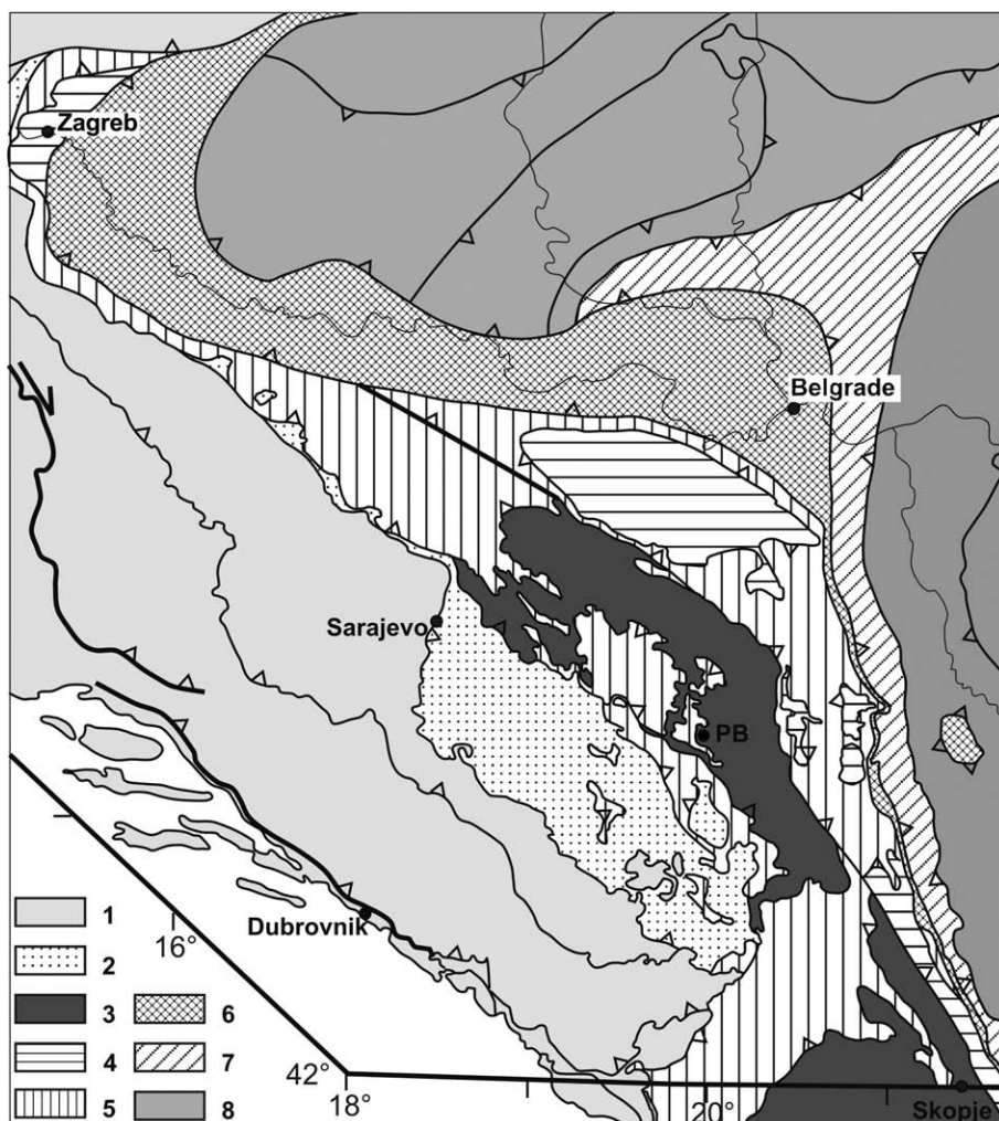
Fig. 2 - Tectonic sketch of the Dinarides (after Schmid et al., 2006), indicating the studied locality. The units mapped are, from external to internal: 1) External Dinarides (without subdivisions); 2) East Bosnian - Durmitor Unit; 3) Drina Ivanjica Unit (parallelized with the Korab Unit of Albania or the Pelagonian Massif of Greece, part of the Internal Dinarides); 4) Jadar and Kopaonik blocks (part of the Internal Dinarides); 5) Dinaric and Western Vardar ophiolites (parallelized with the Mirdita ophiolites of Albania, obducted onto the internal Dinarides in Jurassic times); 6) Sava Belt (Paleogene suture zone); 7) Eastern Vardar Ophiolites; 8) "European" units (Tisza-Dacia and Carpatho-Balkan). PB-Pavlovića Brod.
